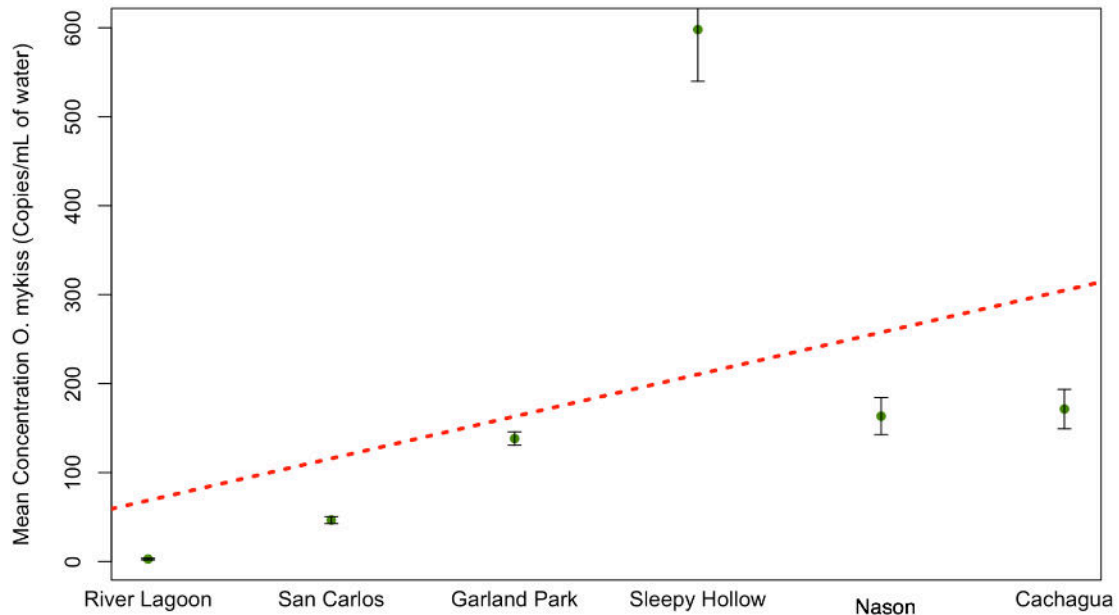
Figure 9. Concentration of O. mykiss eDNA concentration, sites ordered according to their river mile, with River Lagoon being closest to the river mouth. Bars indicate 95% confidence interval. (Spearman's rank correlation, r_s=0.83 , n=6 , S=6 , p=0.058 ).
