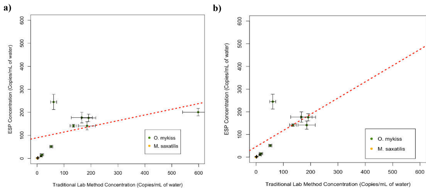
Figure 6. Mean copy numbers of both O. mykiss and M. saxatilis recorded at each sample site. a) all site locations included. b) Sleepy Hollow site omitted. Horizontal bars indicate 95% confidence interval for traditional lab methods, vertical bars indicate 95% confidence interval for the 3G-ESP. Red dotted line indicates the line of best fit.
