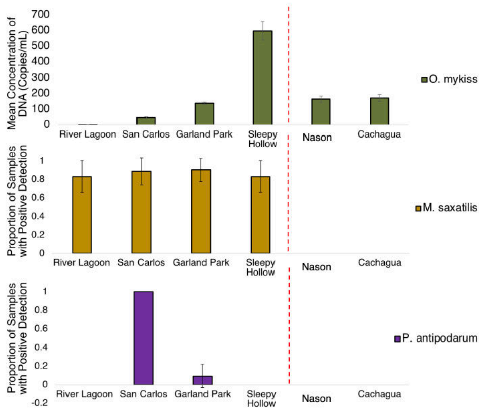
Figure 8. Distribution of species along the Carmel River. Sites ordered according to their river mile, with River Lagoon being closest to the river mouth. Red dashed line indicates historic location of the San Clemente dam.
