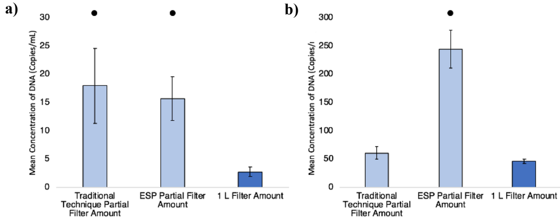
Figure 5. Mean copy numbers of O. mykiss captured based on quantity of water filtered. a) River Lagoon site; mean traditional partial filter amount = 400 mL, mean ESP partial filter amount = 377 mL. b) San Carlos site; mean traditional partial filter amount = 383 mL, mean ESP partial filter amount = 377 mL. Dots above bars indicate significant difference to the 1 L filter amount. Bars indicate 95% confidence interval for traditional lab methods.
