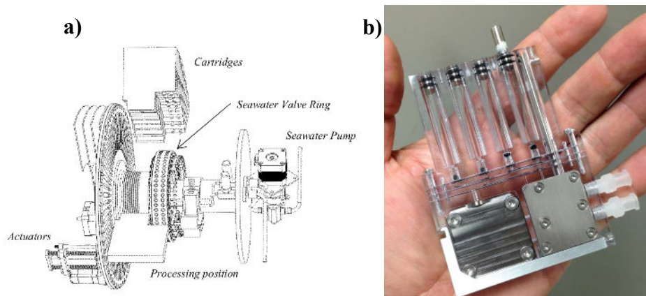
Figure 1. a) exploded diagram of 3G-ESP instrument b) close up image of a single cartridge. Adapted from Pargett et al. 2015.
