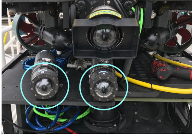
Figure 2: Close up of MiniRov showing stereo camera pair (circled in blue).
