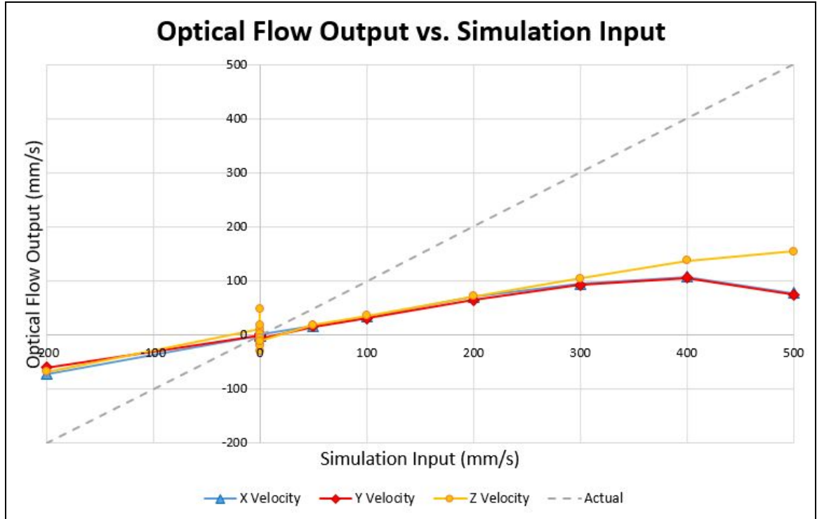
Figure 4: Graph showing the uncorrected optical flow results vs. the simulation input. Each point represents the average velocity output over a single simulation at constant velocity along either the X, Y, or Z axis. The gray line represents the ideal output (output exactly matching simulation input.)
