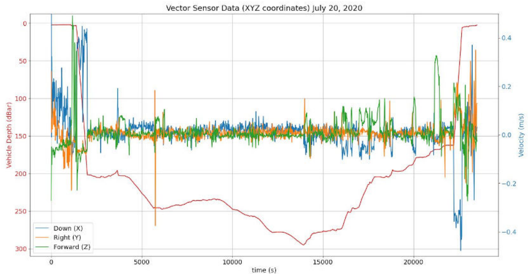
Figure 11: Speed and depth measurements over time of the MiniROV during a July cruise. Note that the velocity scale is shown on the right side, in m/s.
