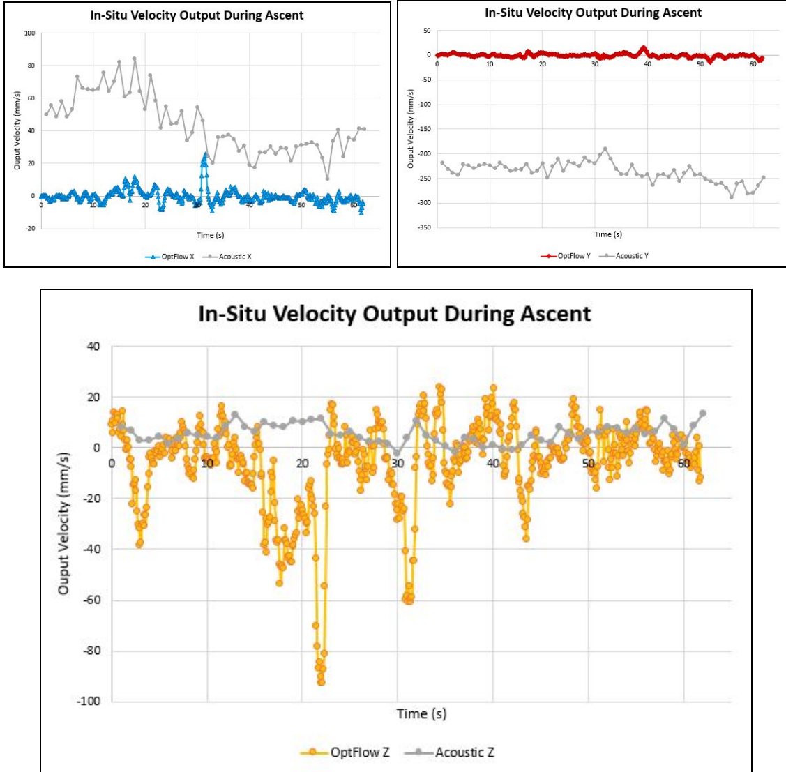
Figure 10a, 10b, 10c: optical flow and acoustic ADV X (a), Y (b), and Z (c) velocity results over time for a period of time when the ROV was ascending very quickly.
