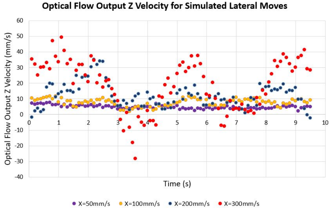
Figure 5: Optical flow Z output over time for four simulations with zero Z velocity input and various lateral speeds.
