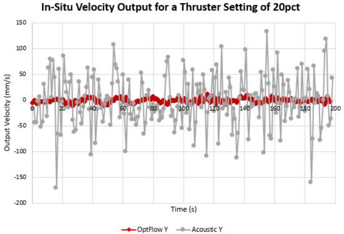
Figure 8: optical flow and acoustic ADV Y velocity results over time for a period of time when the thruster setting was 20 percent.
