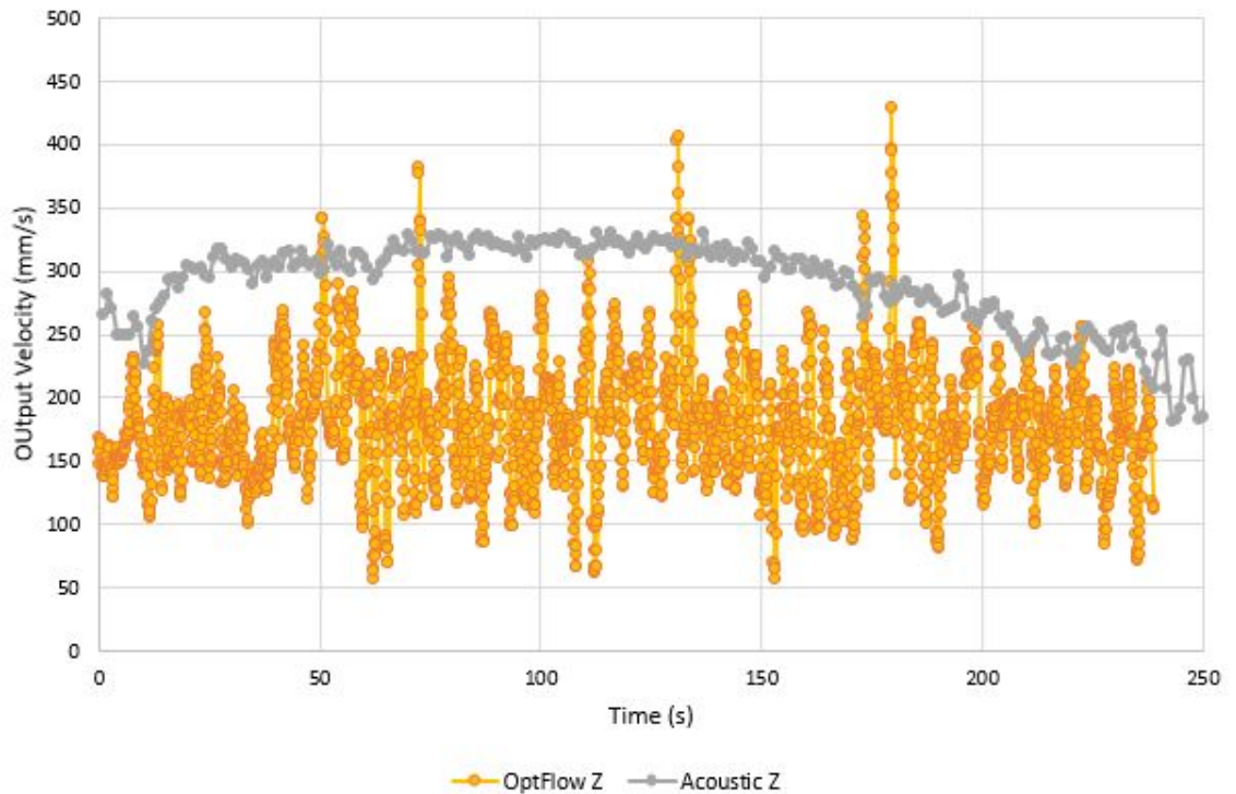
Figure 9: optical flow and acoustic ADV Z velocity results over time for a period of time when the Thruster setting was 50 percent.
