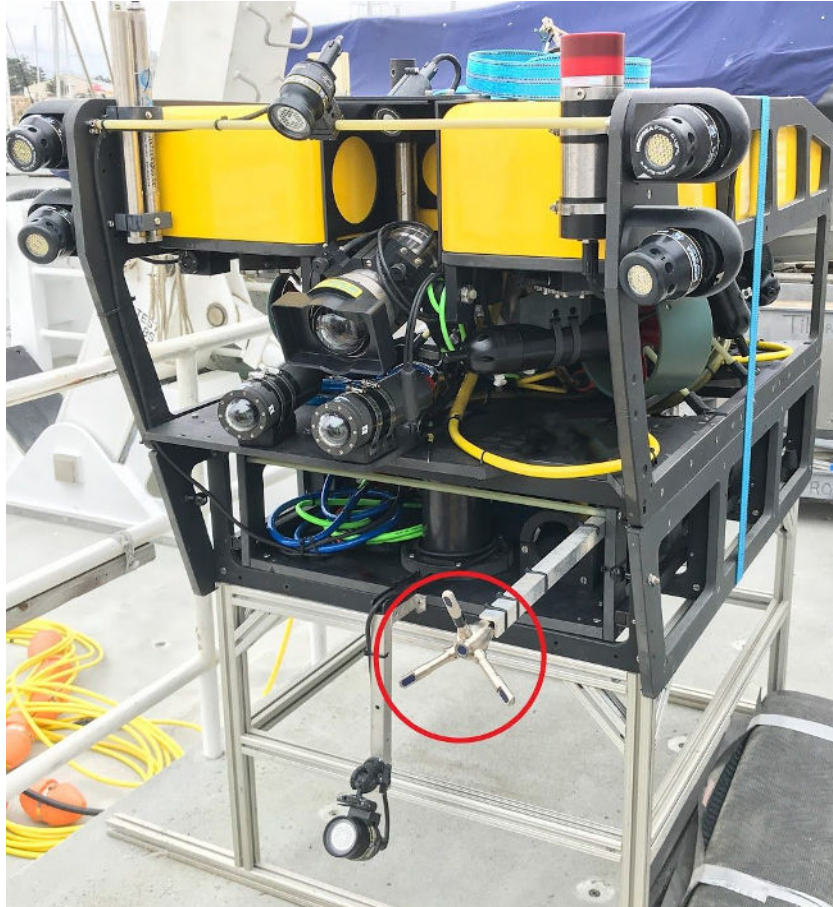
Figure 1: MiniROV with ADV circled in red.
