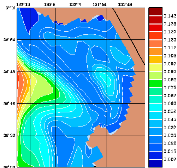
Salinity (PSU) at Level 1
