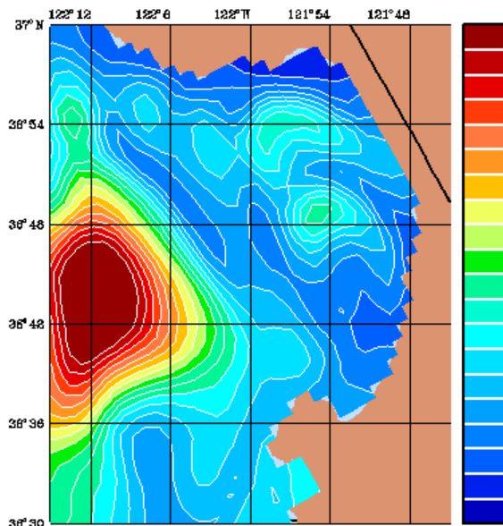
Temperature (°C) at Level 1
