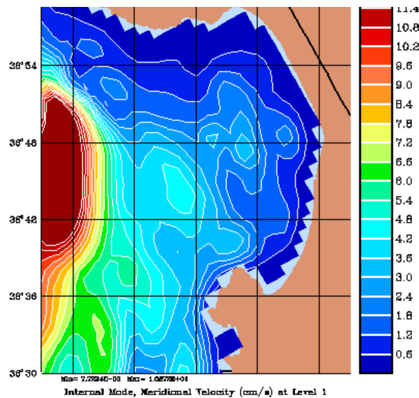
Internal Mode, Meridional Velocity (cm/s) at Level 1
