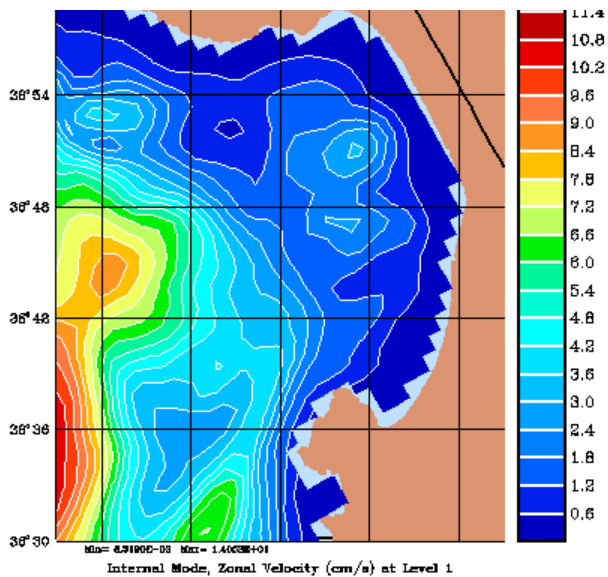
Internal Mode, Zonal Velocity (cm/s) at Level 1
