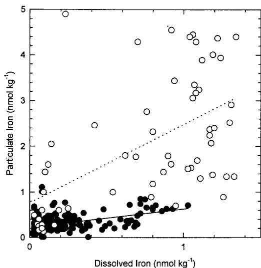
Fig. 11. Particulate iron versus dissolved iron. Data from 4 stations near the continental margin are shown as open circles (VERTEX V, Stations 1 and 2 near the California margin, VERTEX VII, Station 8 near the Alaska margin and Station 30 over the continental slope in the Ross Sea). The remaining stations are shown as closed circles. The dashed line is a least squares fit to the open circles and the solid line is a fit to the closed circles.
