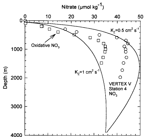
Fig. 13. A model profile of nitrate calculated with eddy diffusion coefficients of 0.5 and 1 \text{cm}^2 \text{s}^{-1} . The vertical profiles of nitrate and oxidative nitrate ( 15\times apparent oxygen utilization) at VERTEX V Station 4 in the North Pacific are shown for comparison.
