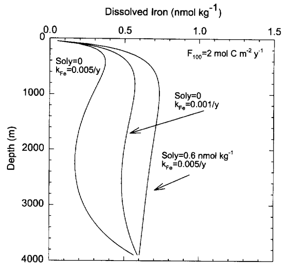
Fig. 15. Model calculation profiles of dissolved iron with the apparent solubility set to zero and scavenging rate constants of 0.005 \text{ yr}^{-1} and 0.001 \text{ yr}^{-1} and an F_{100} of 2 \text{ mol C m}^{-2} \text{ yr}^{-1} . The standard model calculation with a solubility of 0.6 \text{ nmol Fe kg}^{-1} is shown for comparison.
