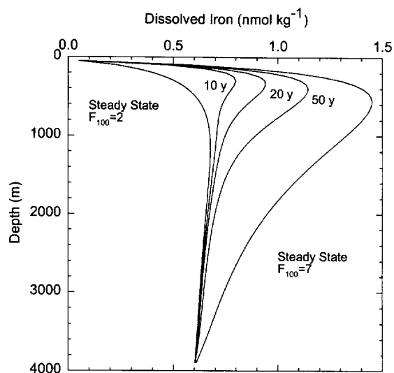
Fig. 16. Change in iron concentrations calculated at 10, 20 and 50 yr after a step change in the value of F_{100} from 2 to 7 \text{ mol C m}^{-2} \text{ yr}^{-1} . The steady state iron profiles for each value of F_{100} are shown as well.
