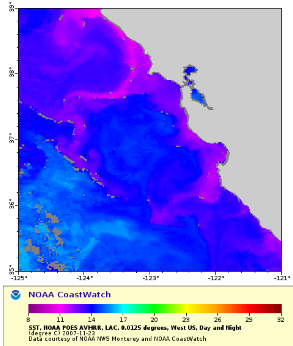
Figure 8. Advanced Very High Resolution Radiometer (AVHRR) satellite image of sea surface temperature ( ^{\circ} C) of the area of operation during the PaCOOS cruise of November 2007. The image was taken on 23 November 2007.
