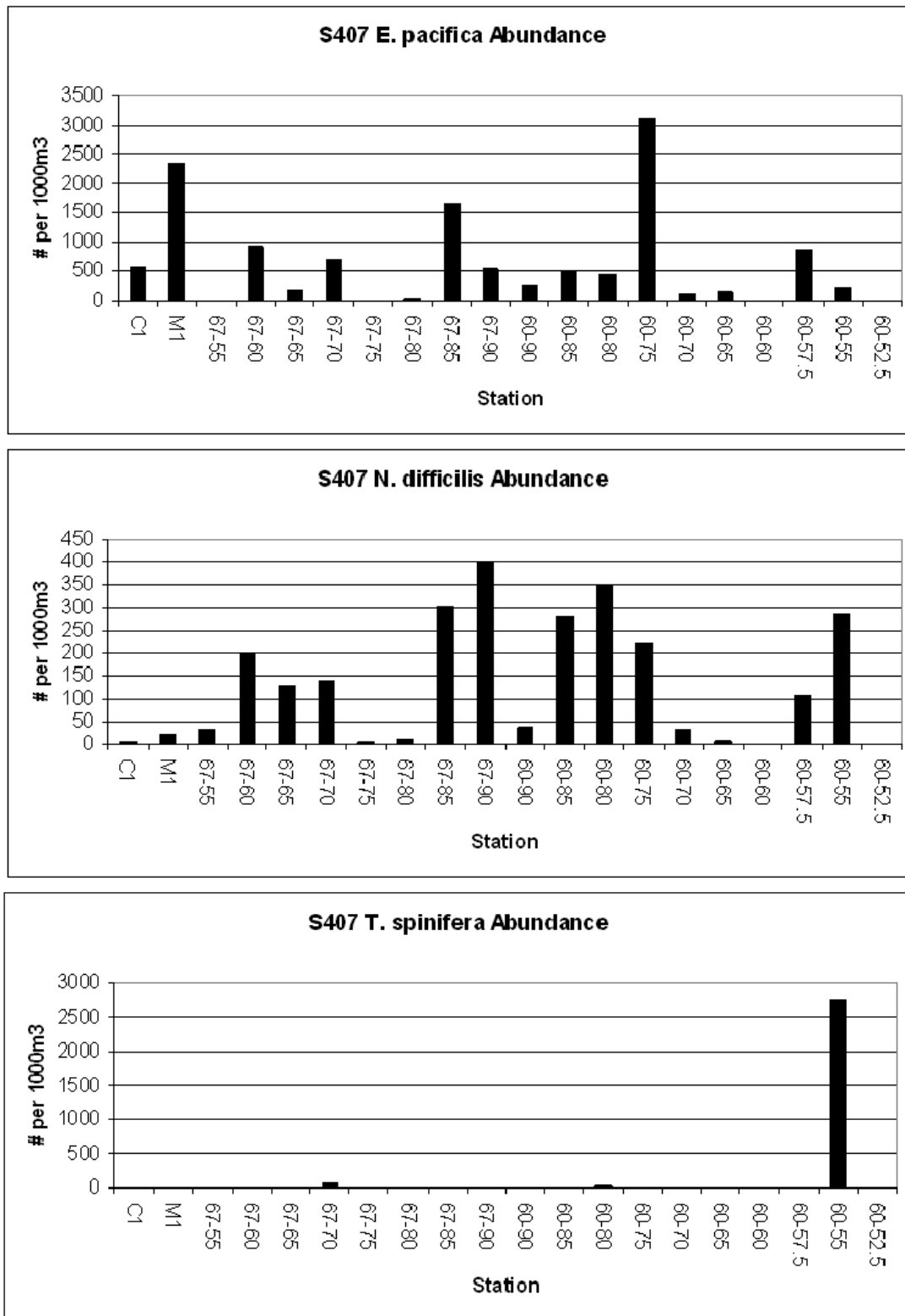
Figure 6: Krill abundance for the three most common species collected at stations sampled along CalCOFI lines 67 and 60 during the PaCOOS cruise of November 2007. Top = Euphausia pacifica , middle = Nematoscelis difficilis , and bottom = Thysanoessa spinifera . Note that the y-axis scale differs for each graph.
